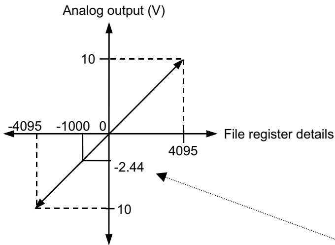
<Relation of file register details and analog output voltage>
